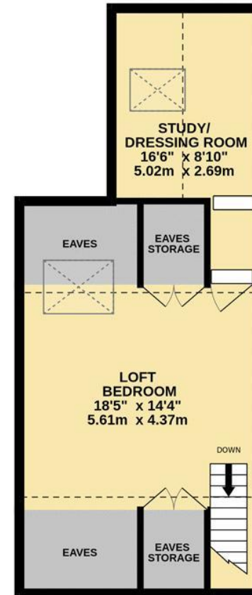
2ND FLOOR 437 sq.ft. (40.6 sq.m.) approx.
